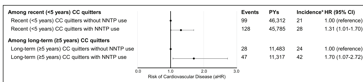
Figure 4. Association of changes in CC and NNTP use habits with cardiovascular disease risk after propensity score matching among CC quitters.
